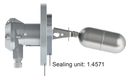
Slip-on Flange: Carbon steel P265GH zinc galvanized and passivated
