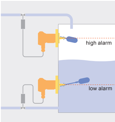
max/min limits
