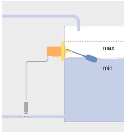
pneumatic control
